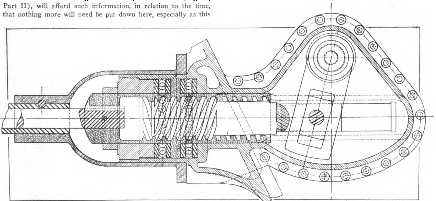
Fig. 36.—Screw and nut design showing one way of transforming the motion as used in exacting truck service.
